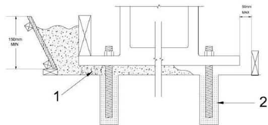
1. Base Plate Grouting, 2. Bolt Pocket Grouting
